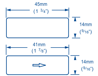
FV1227 SIDE VIEW
