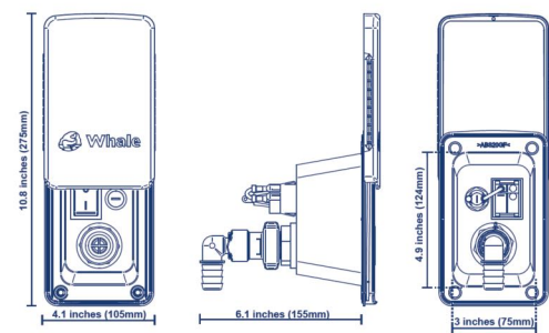
4 IN 1 FITTING
