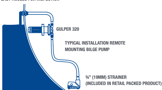
EASY ACCESS FOR INSPECTION
