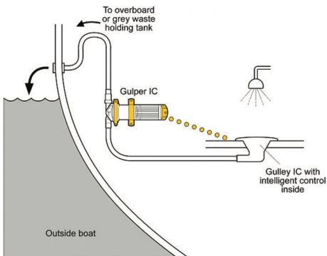
TYPICAL INSTALLATION
