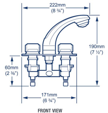
MIXER FAUCET STANDARD OUTLET
