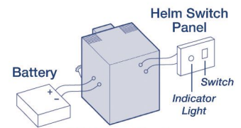
12V Water Heater SIMPLIFIED INSTALLATION
