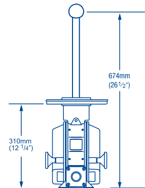
BP3020 SIDE VIEW
