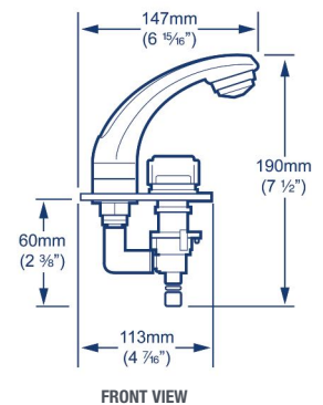
SINGLE FAUCET COLD ONLY
